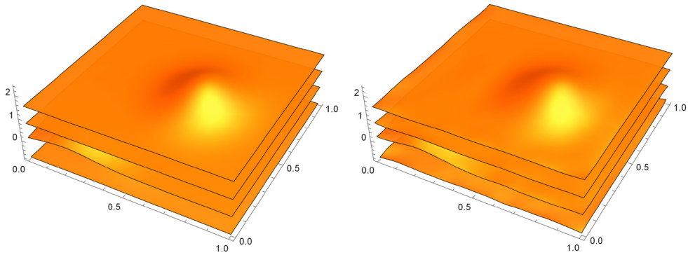
Fig. 1. From left to right, the original fuzzy function and its approximation for nctrs = 81 , np = 100 , \tau = 1e - 9 and \varepsilon = 1 .
