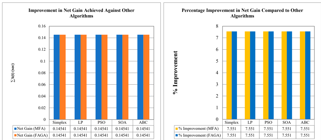
Figure 3. Net gain improvement of proposed algorithms compared to other algorithms for IEEE 3-bus system (LP formulation).
