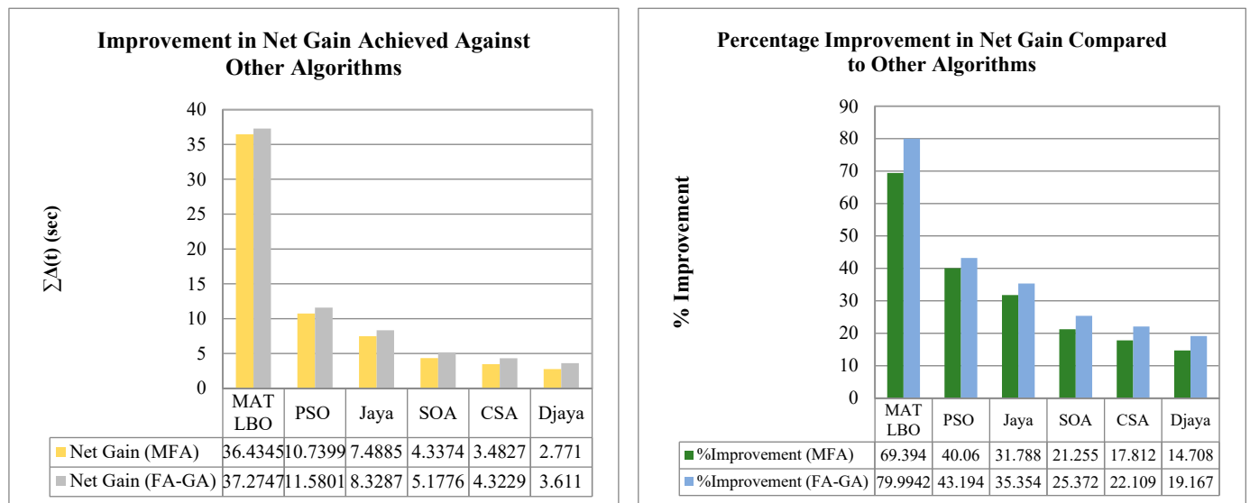
Figure 13. Improvement in net gain of the proposed algorithms compared to other algorithms for IEEE 15-bus system (NLP formulation).
