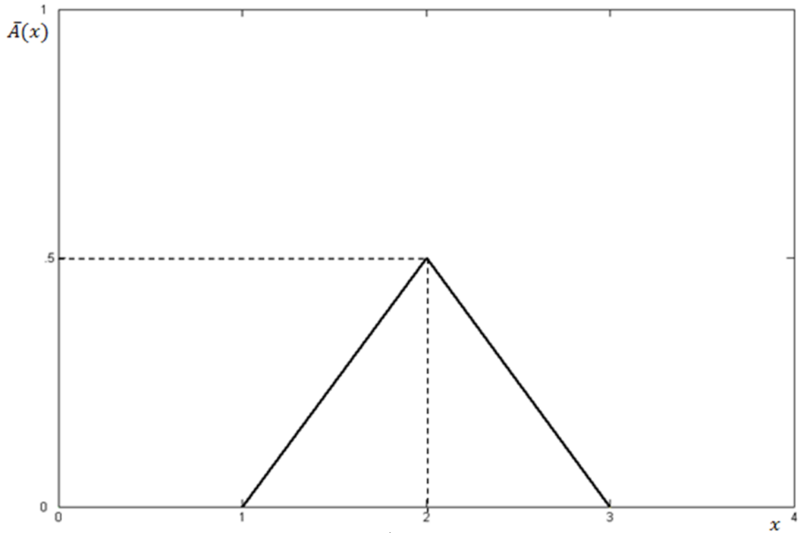
Figure 1.4.1 Fuzzy Set
